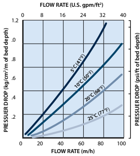
Fig. 1 PRESSURE DROP VS FLOW RATE
