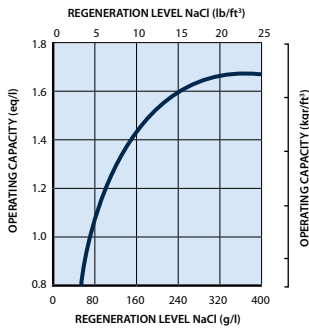
Fig. 3 OPERATING CAPACITY, C g
